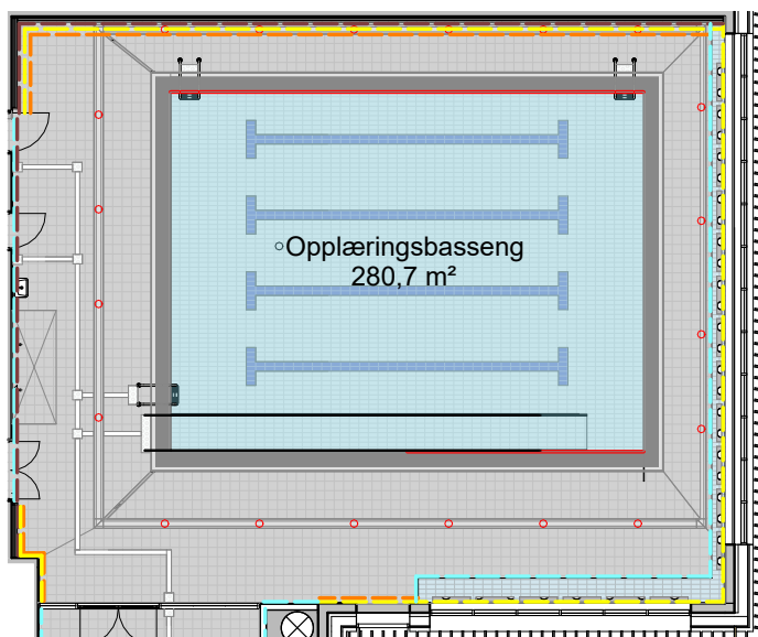
Plan diagram
